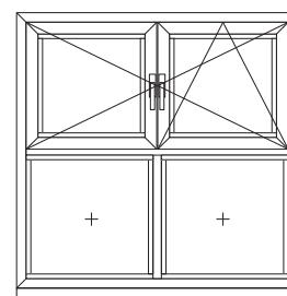
A pivoting casement, a pivoting / tilt casement and two fixed casements
