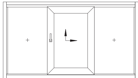
One operating sash (centre), opening right
