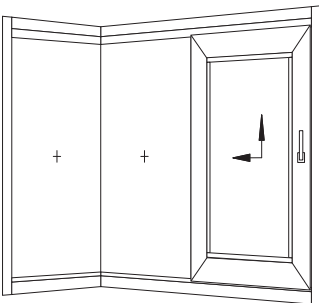
90°-fully glazed corner, one operating sash, opening left
